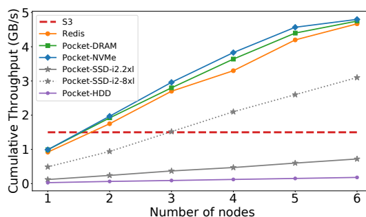
Figure 6: Total GB/s for 1MB requests from 100 lambdas
