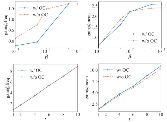
Figure 13: Impact of \beta and r on the defense effectiveness of OC against M2GA for PCKV-UE on TalkingData.
