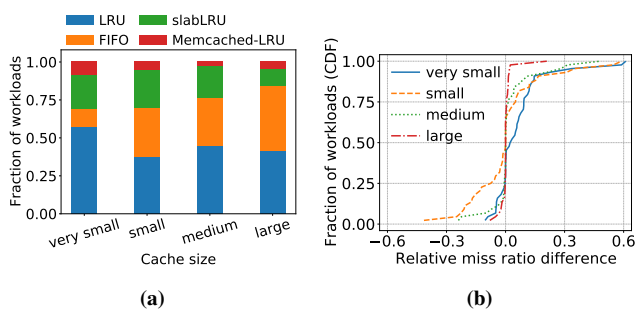
Figure 15: a) The best eviction algorithms under different sizes. b) The relative miss ratio difference between FIFO and LRU under different sizes. Positive region shows FIFO is worse.
